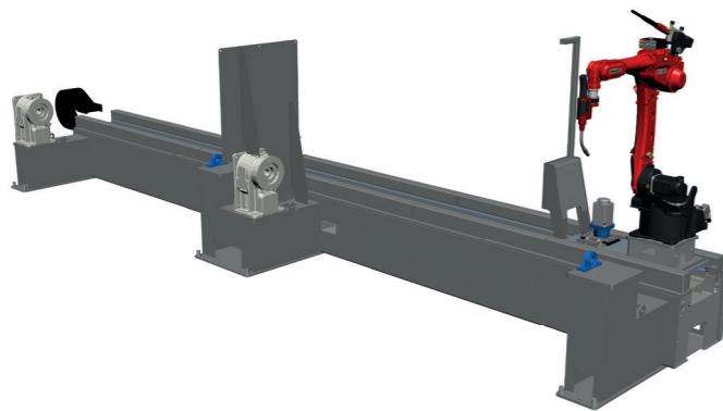
TRACK-FRAME-E
