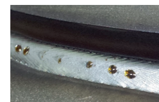
Hyperdip-puls-process
