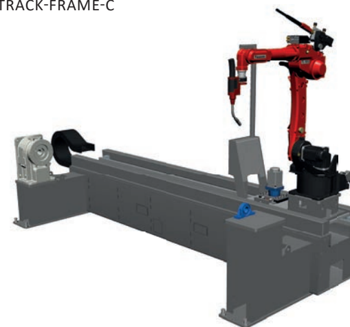
TRACK-FRAME-C
